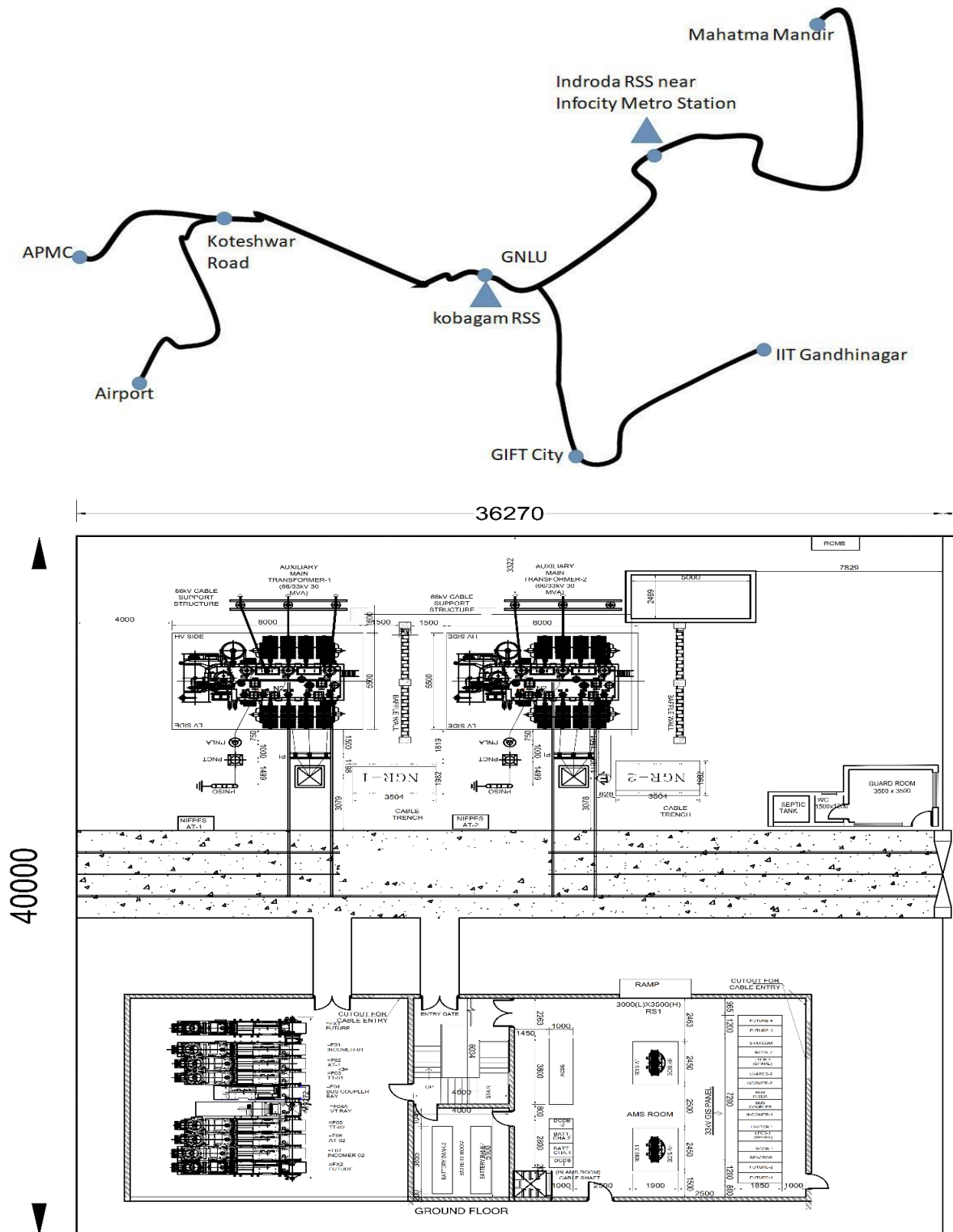
Figure 10.1: Layout of a Typical Receiving Substation equipped with High Voltage Gas Insulated Switchgear (GIS)
