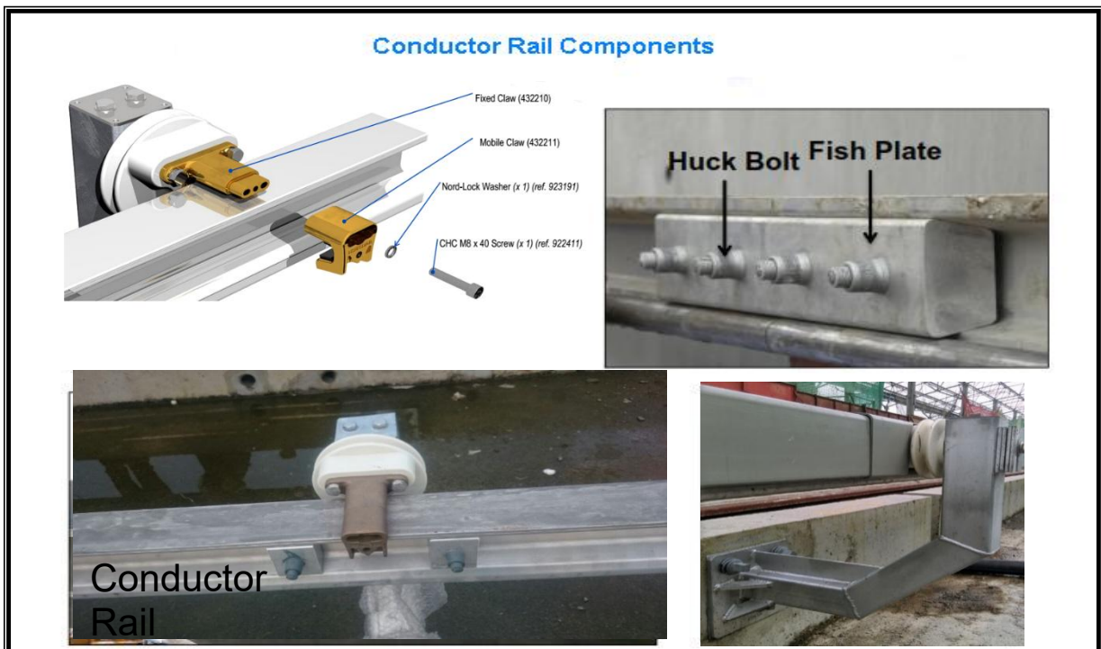
Figure 10.6: 750V dc Third Rail Current Collection System
