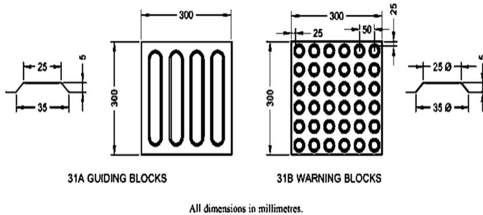
Figure 13-12: Guiding Paver (Source*National Building Code-2016)
