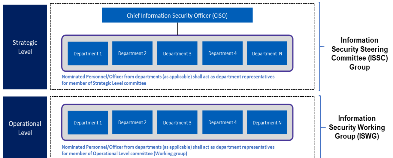
Fig. 22.1: Governance Structure
