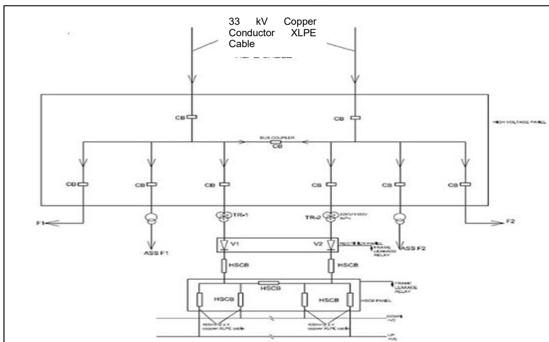
Figure 10.7: Schematic Diagram of DC Traction Substation (TSS) at Metro Stations
