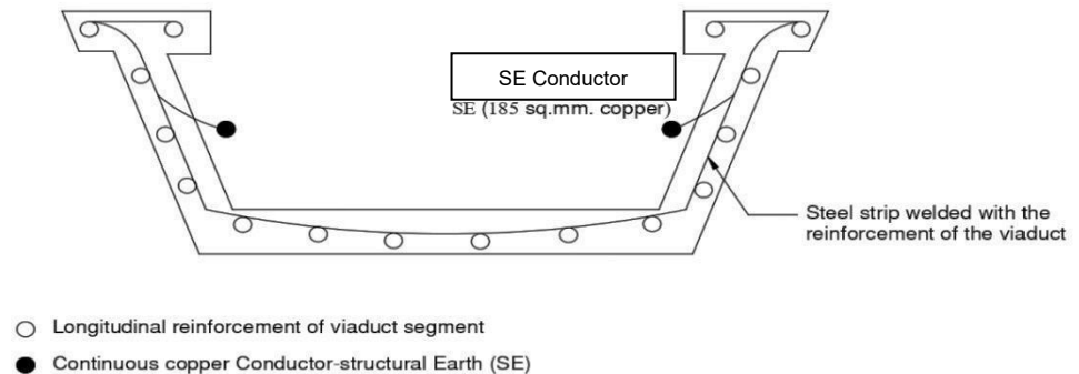
Figure 10.10: Connection of SE Conductor to Steel Reinforcement of Viaduct Segment
