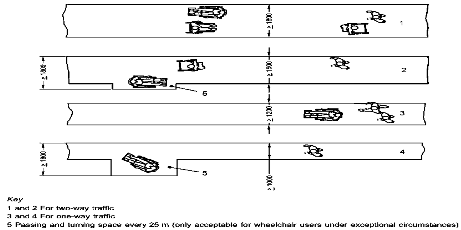
FIG. 26 DIFFERENT SURFACE WIDTHS OF THE PATH DEPENDING ON TRAFFIC
