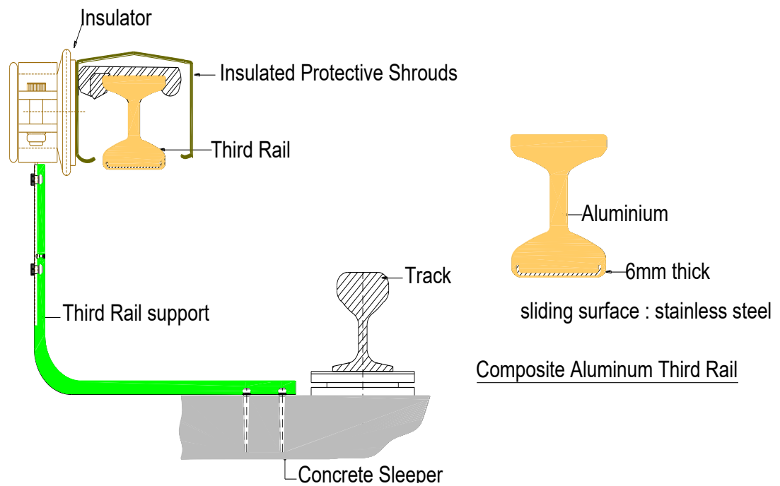
Figure 0.1 : Depot Third Rail Current Collection System
