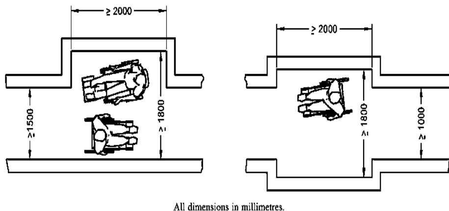
FIG. 27 EXAMPLES FOR PASSING PLACES FOR WHEELCHAIR USERS
