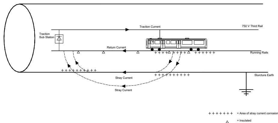
Figure 10.8: DC Traction System: Stray Current Corrosion Concept
