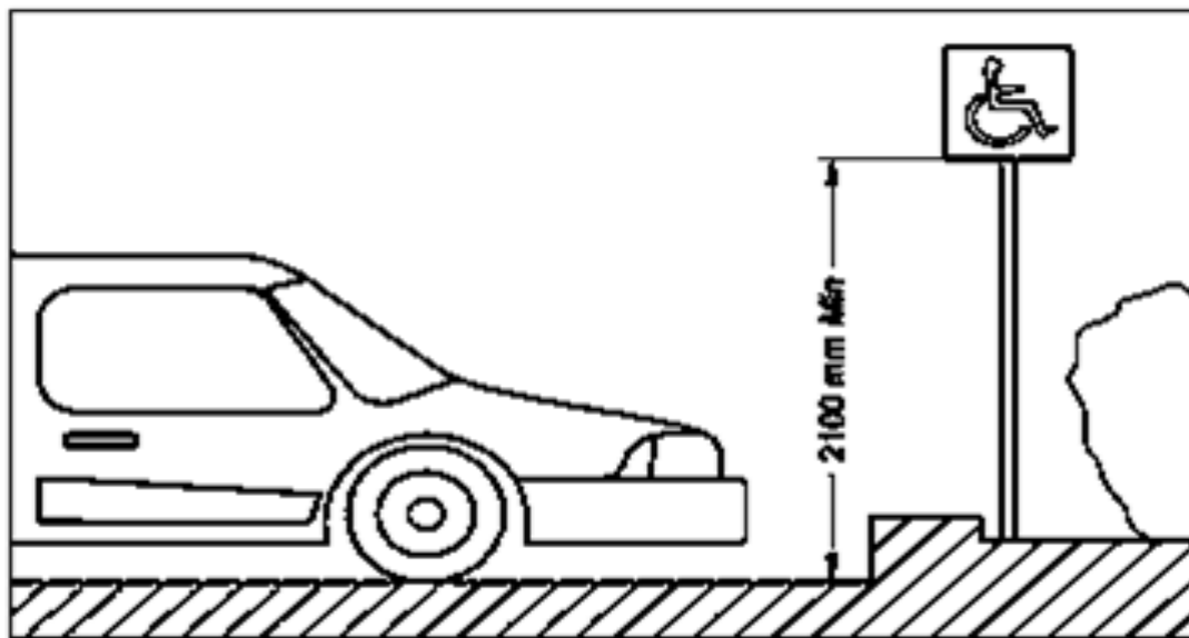
Figure 13-9: (Source*: National Building Code-2016)
