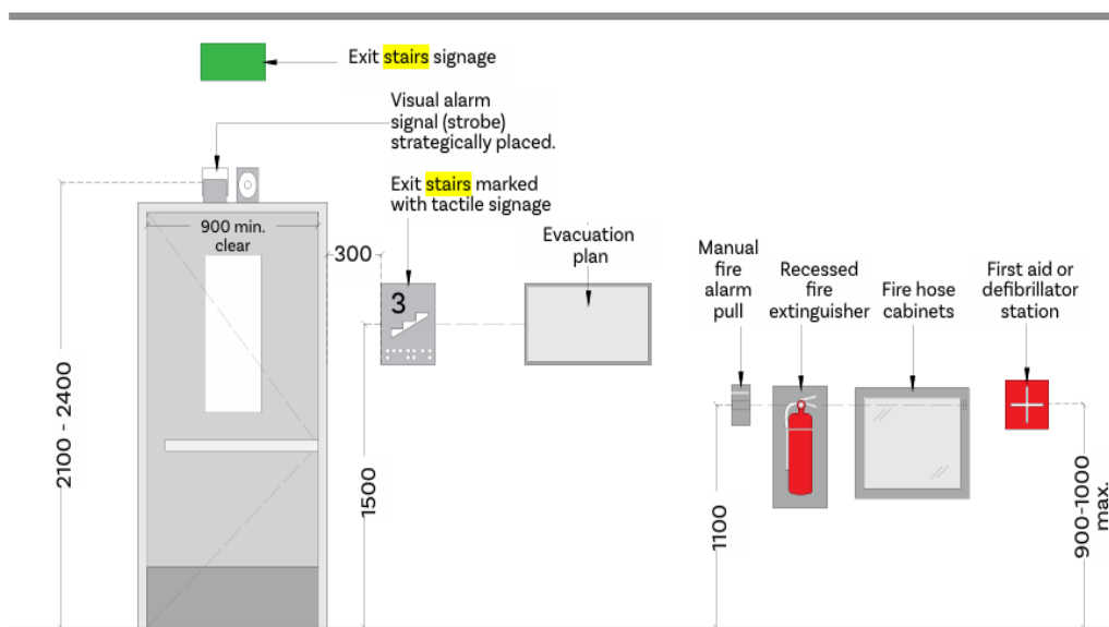
Figure 7.1 Fire Safety and Evacuation Features: Elevation View
