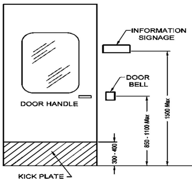
Figure 13-28: Door Layout (Source*: National Building Code -2016)
