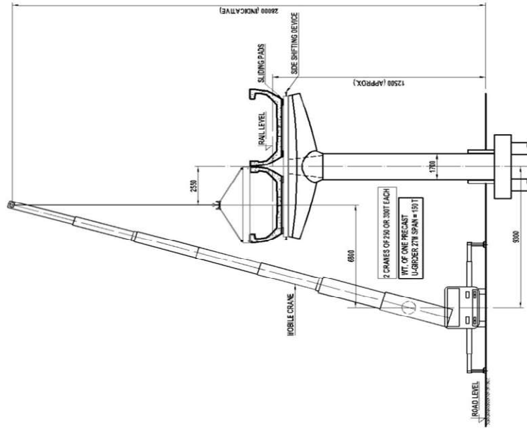
Figure 5.3(b) : Erection of Girder using Crane
