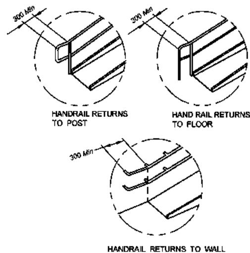
FIG. 54 TYPICAL HANDRAIL EXTENSIONS
