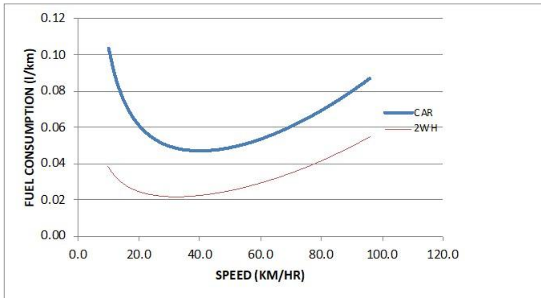
Figure 20.2 Fuel Consumption at Different Speed for Car and Two Wheeler
