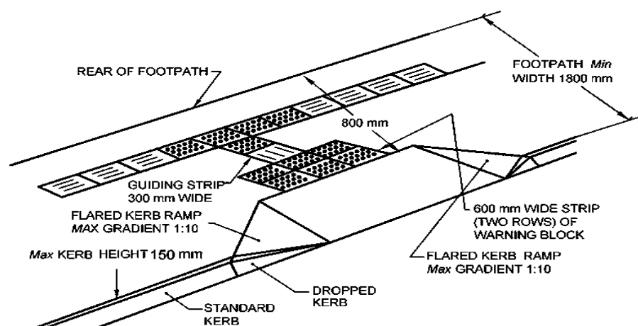
FIG. 29 KERB EXTENSION AT STREET INTERSECTION
