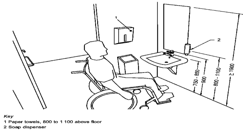
FIG. 81 PLACEMENT OF WASHBASIN AND MIRROR ABOVE THE WASHBASIN WITH DISTANCE OF SANITARY APPLIANCES
