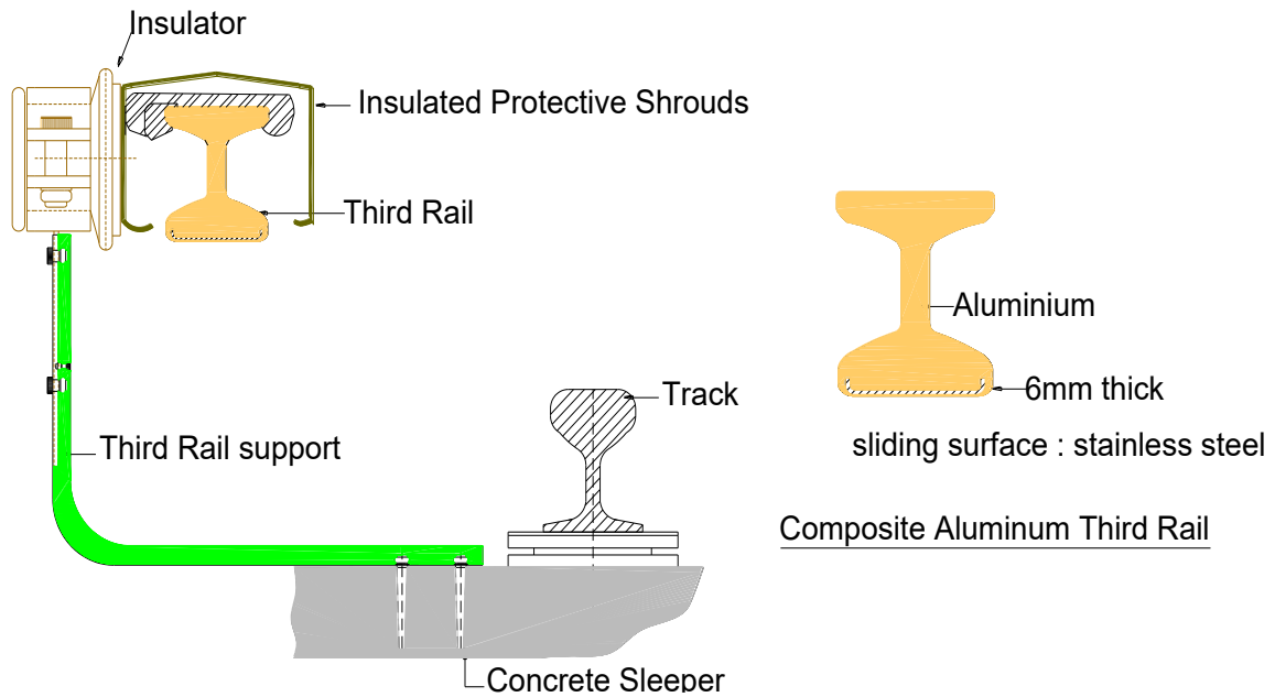
Figure 10.5: Depot Third Rail Current Collection System
