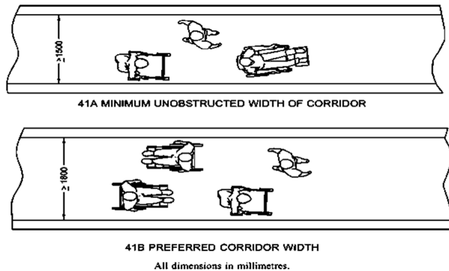
Figure 13-15: Corridor layout (Source*: National Building Code -2016)
