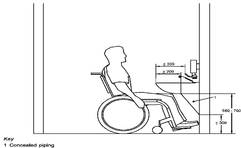
FIG. 82 WASHBASIN WITH KNEE/TOE CLEARANCE
