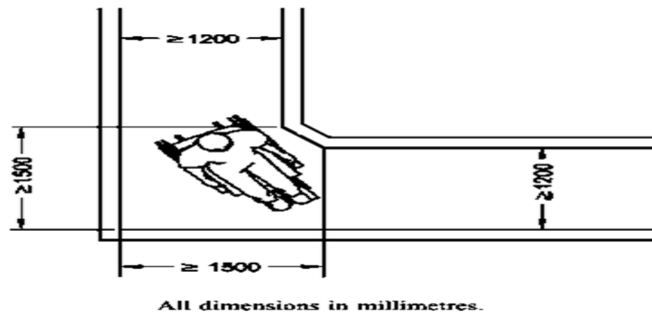
Figure 13-16: Corridor layout (Source*: National Building Code -2016)
