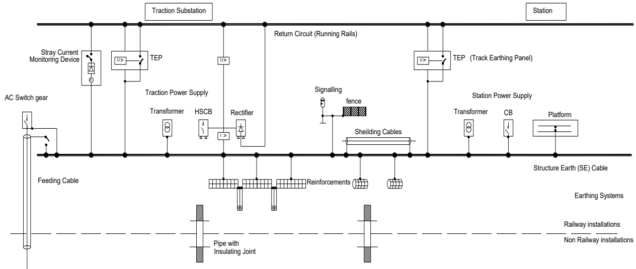
Figure 10.9: Basic Diagram for Earthing, Bonding and Stray Current Protection Measures
