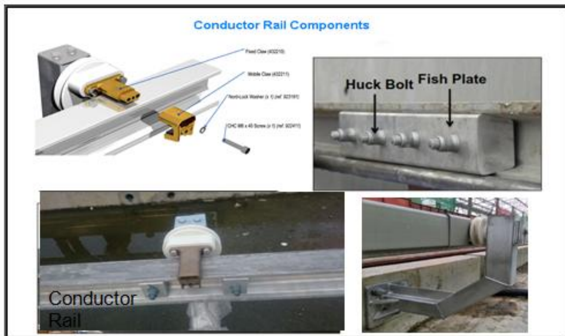
Fig. 0.2 : 750V dc Third Rail Current Collection System
