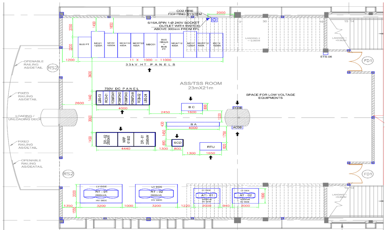
Figure 10.4: Typical Layout of TSS & ASS (Combined)
