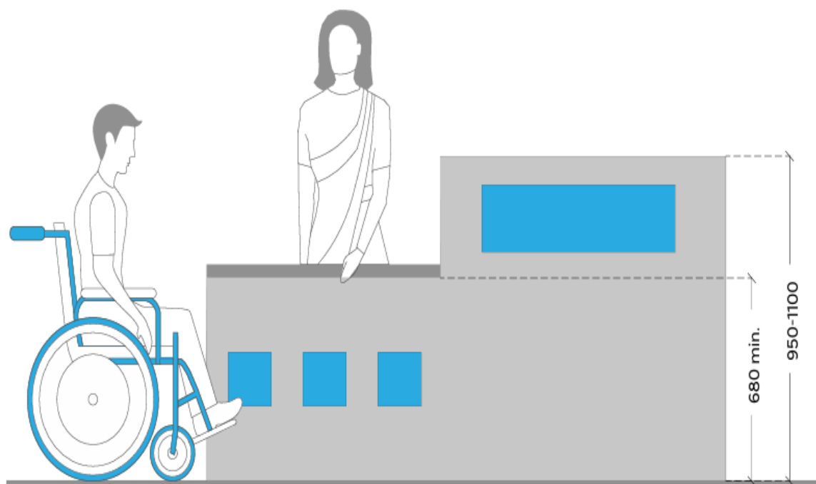
Figure 13-3: Reservation and Information Center
