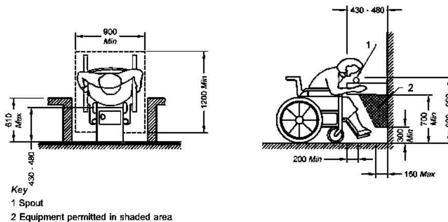
FIG. 70 CLEAR FLOOR SPACE AND KNEE SPACE REQUIREMENT FOR A WALL/POST-MOUNTED DRINKING WATER UNIT
